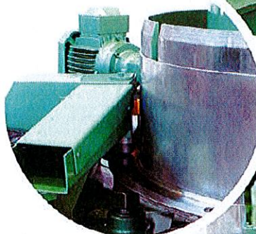
Punching of holes in the flange
