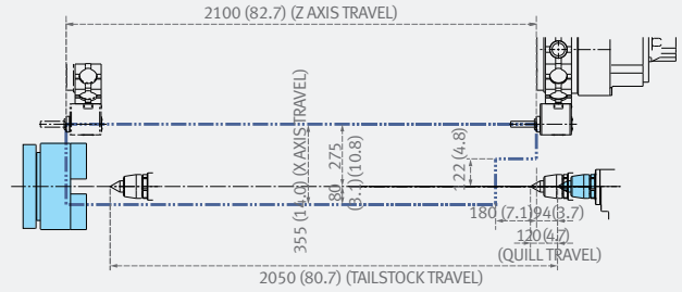
Angular Milling Unit
