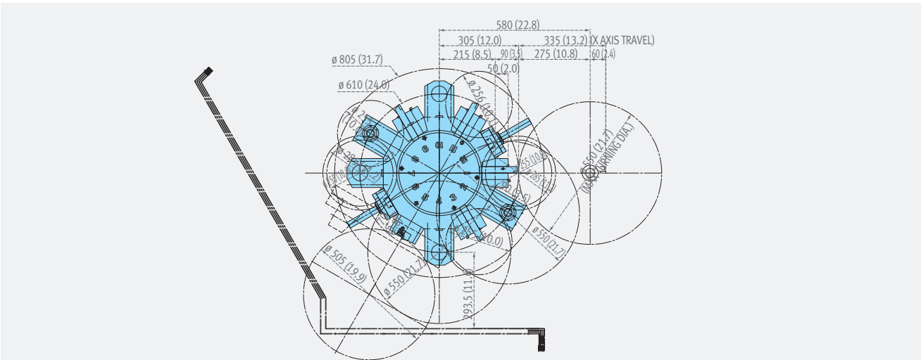
PUMA 5100LY / XLY (12 station)
