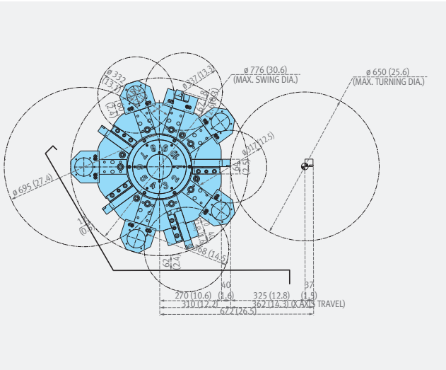
PUMA 5100M (12 station)
