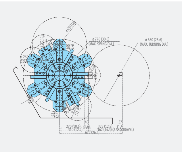
PUMA 5100LY / XLY (12 station)
