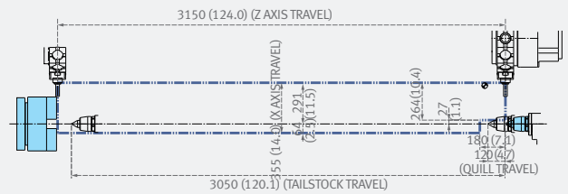
Straight Milling Unit
