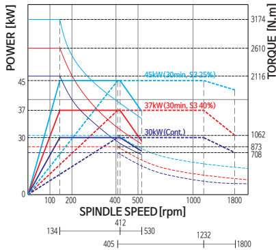
SL 4500XY/LY/XLY (A Type)
