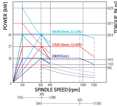
SL 4500XY/LY/XLY (B Type)
