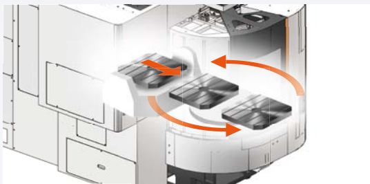
VARIAXIS j-500/5X 2 pallet changer
