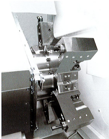
Hydraulic turret
