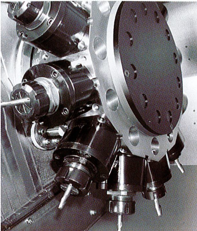
Power turret
